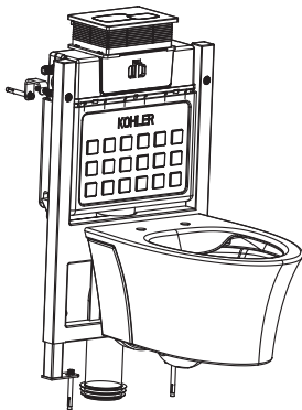
In-Wall Tank With Frame
